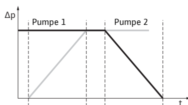
Fig. 16: Pumpeskift
