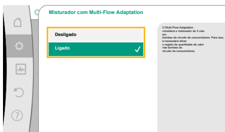
Fig. 60: Misturador com Multi-Flow Adaptation
